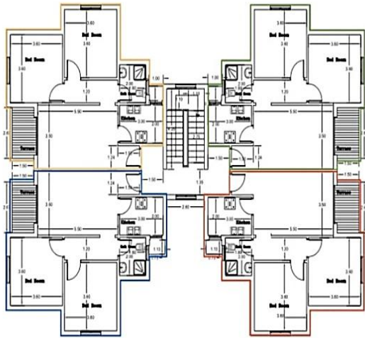
Figure 16. Design proposal for the 70m 2 separating the building mass –regarding the orientation for every unit – avoiding the cross-sections in circulation.
