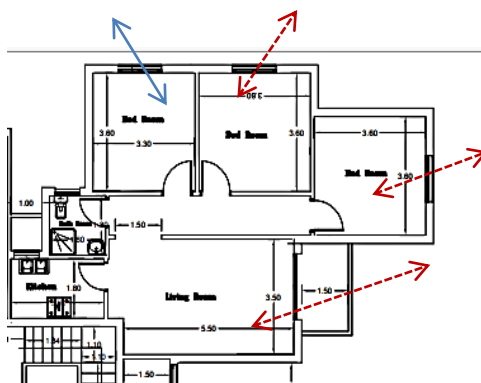
Figure 13. Designing the windows in different orientation allowing good air movement path.
