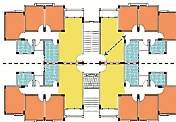
Figure 15. The current area is 90 m 2 and orientation is 2 different directions at maximum.
